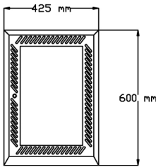
Front Glass Door
